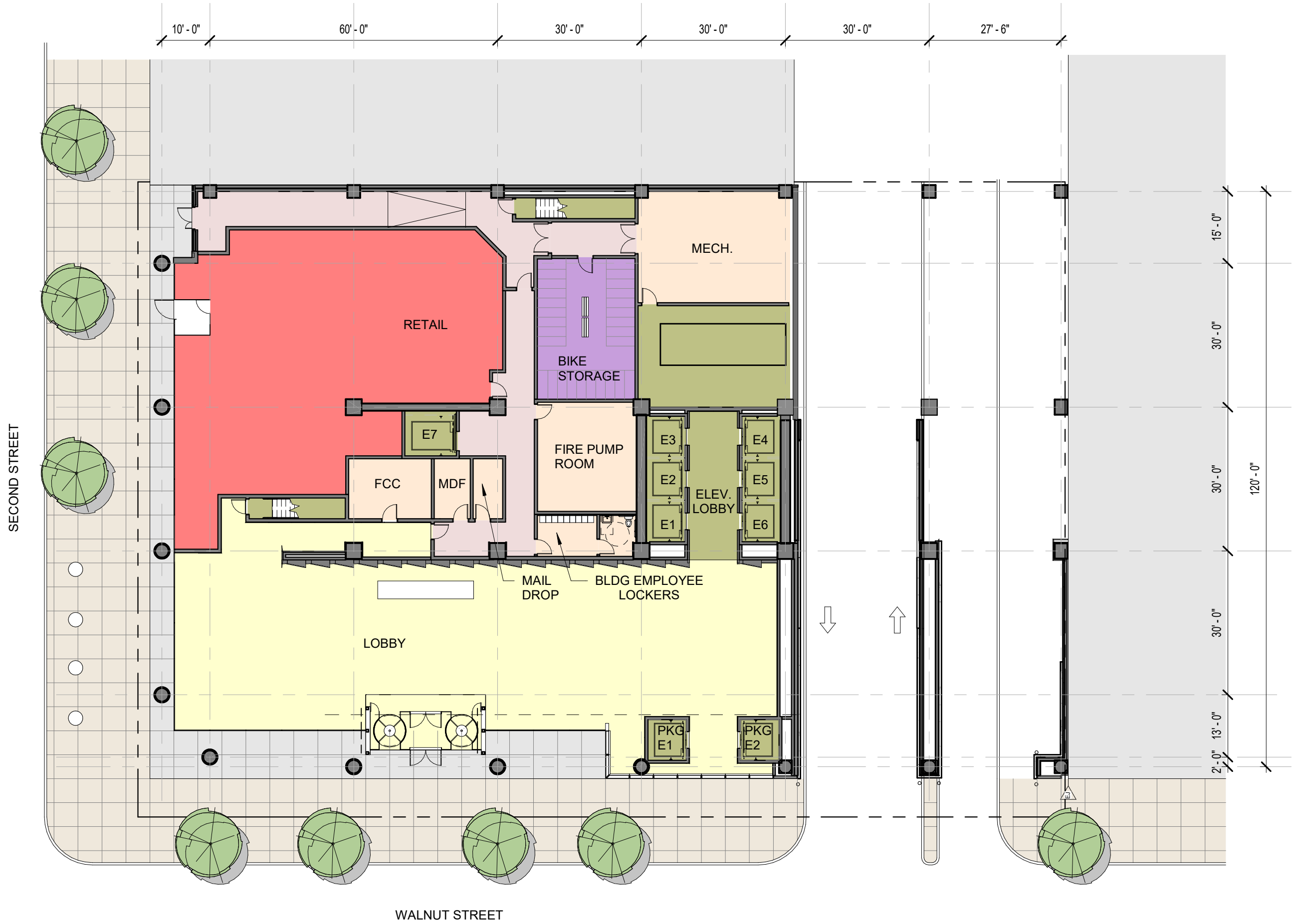
1ST FLOOR PLAN- LOBBY
